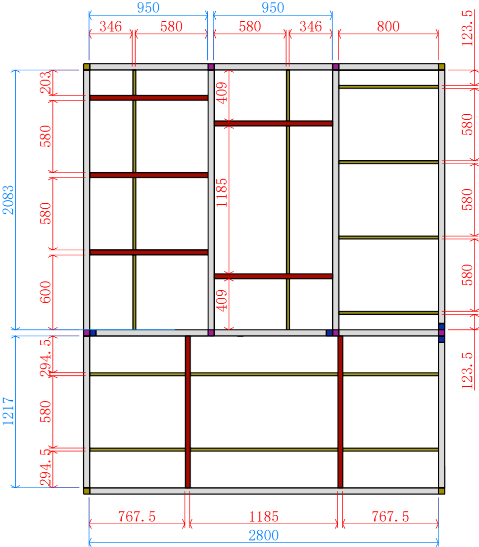
SUB-CEILING GRID ASSEMBLY
