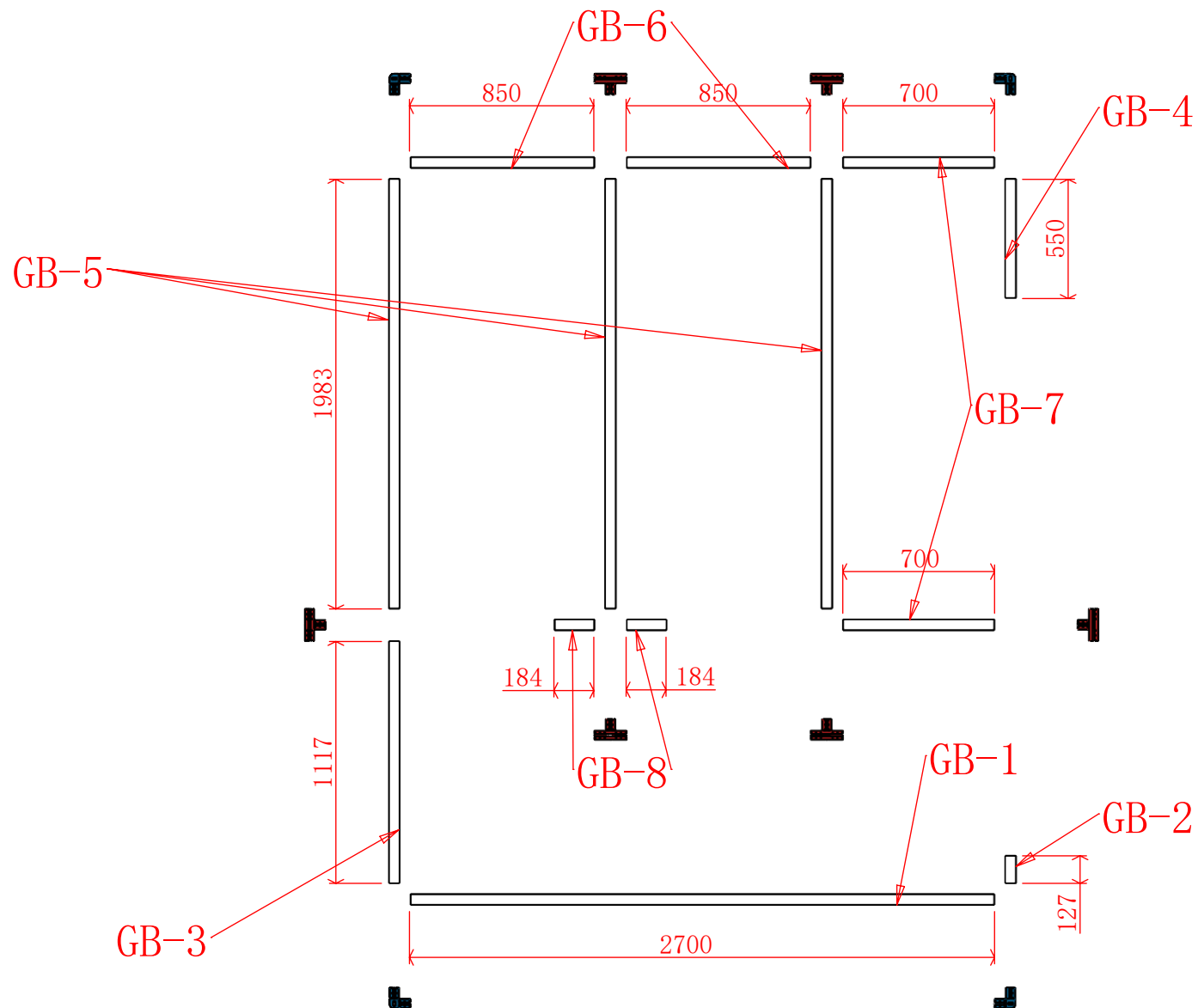
Bottom Frame Assembly
