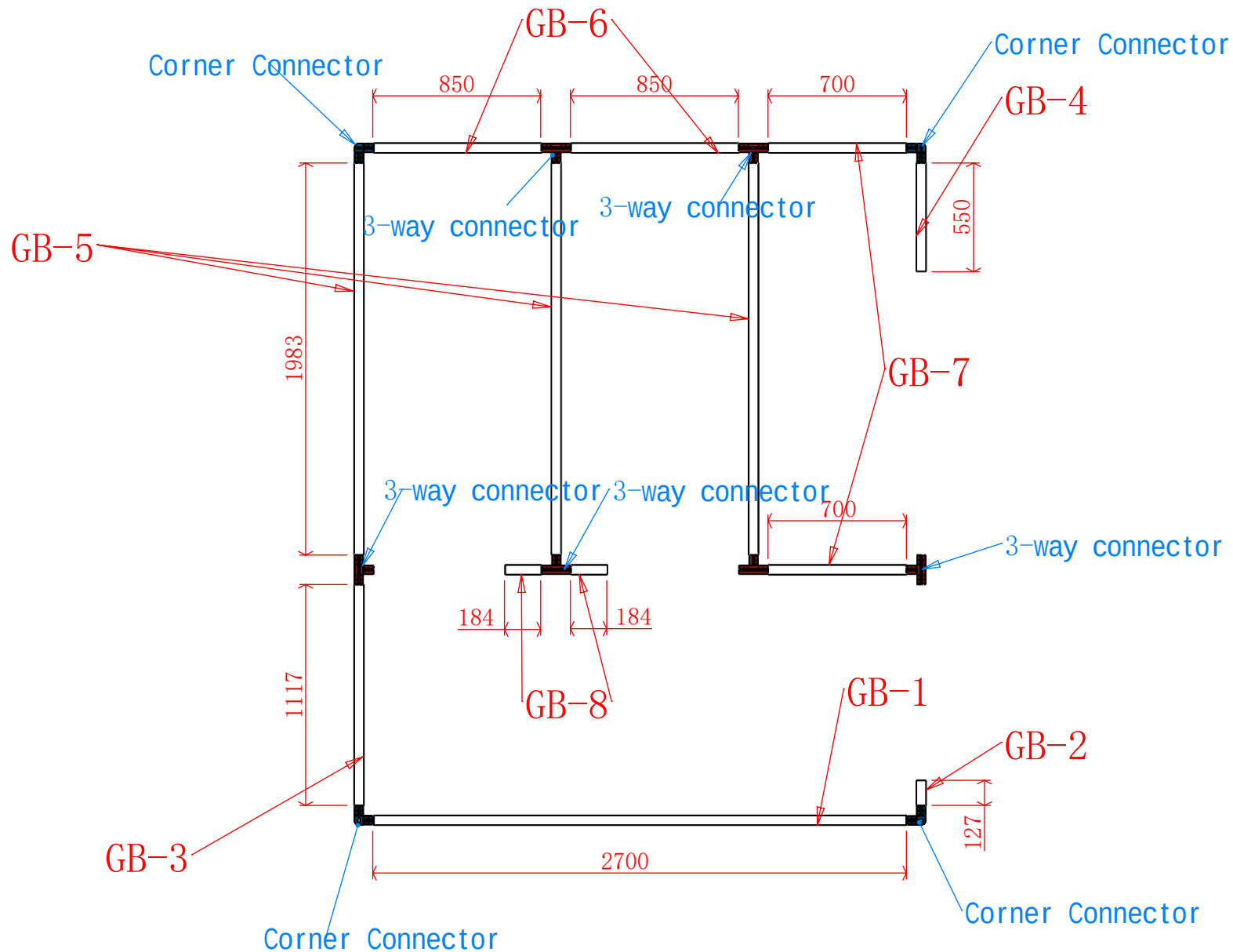
Bottom Frame Assembly
